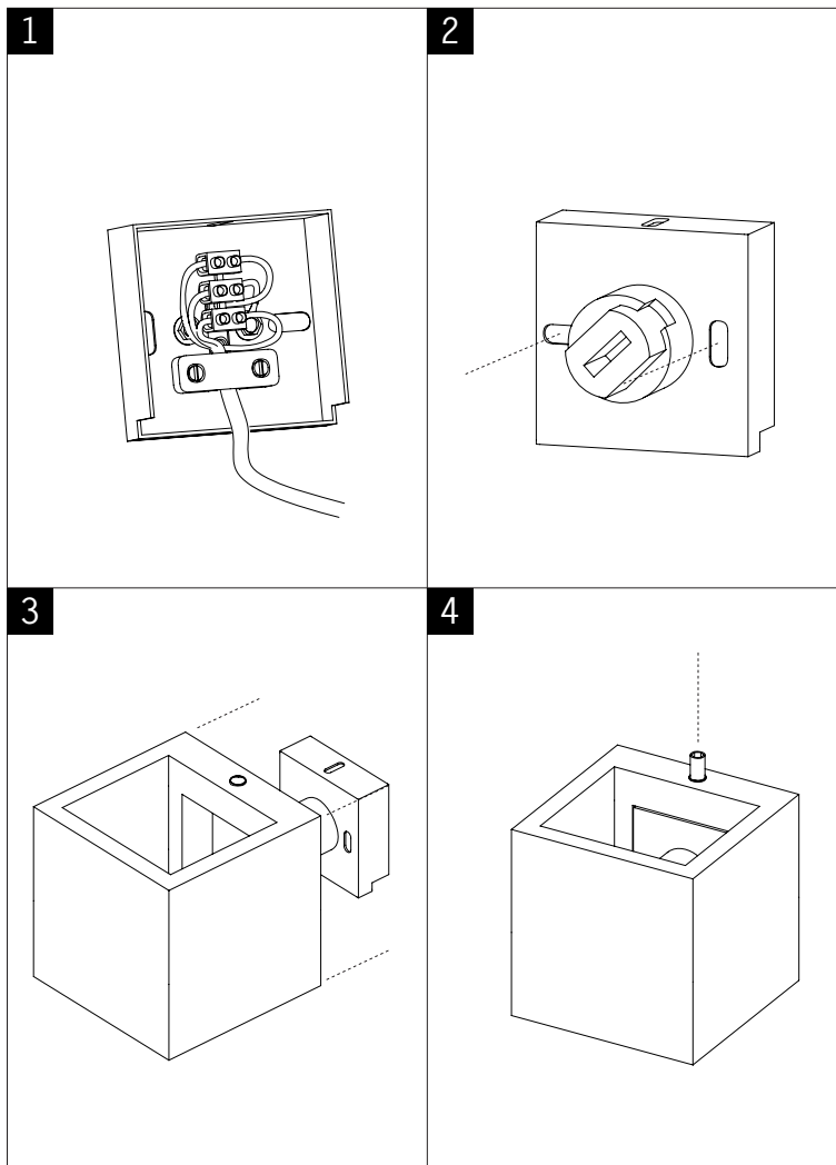
B9 Beton Wandlampe / B9 concrete wall light
