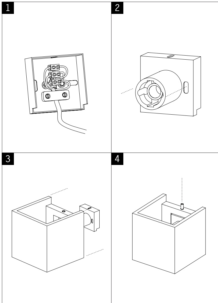
B3 Beton Wandlampe / B3 Concrete wall light
